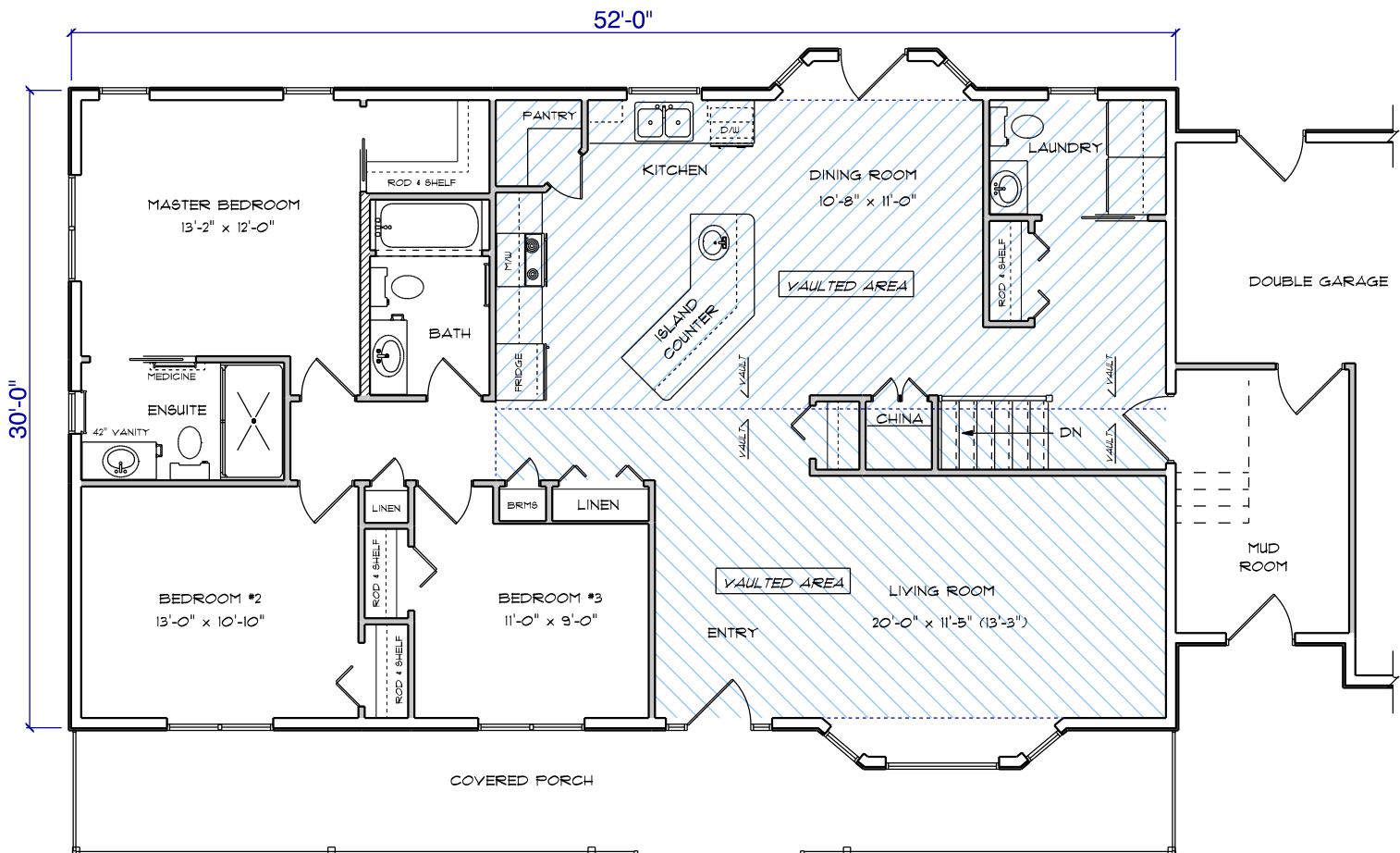
MAIN FLOOR PLAN 1591 SQ. FT.
