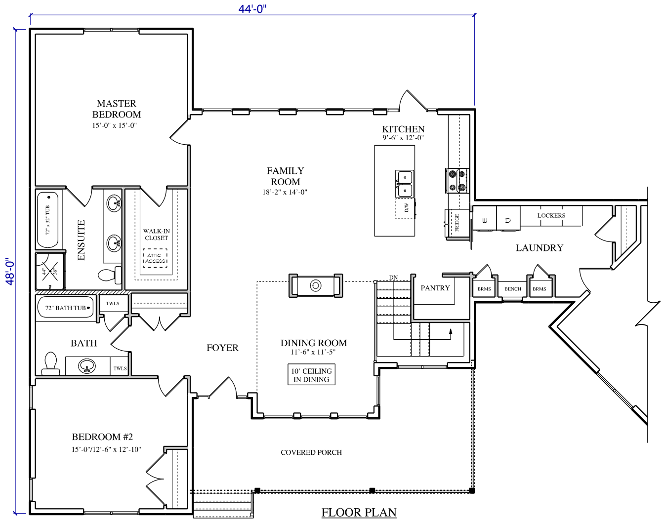
FLOOR PLAN 1710 SQ. FT.
